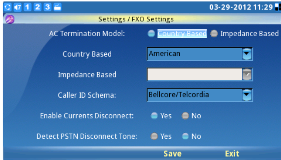
Figure: FXO Port LCD Configuration
