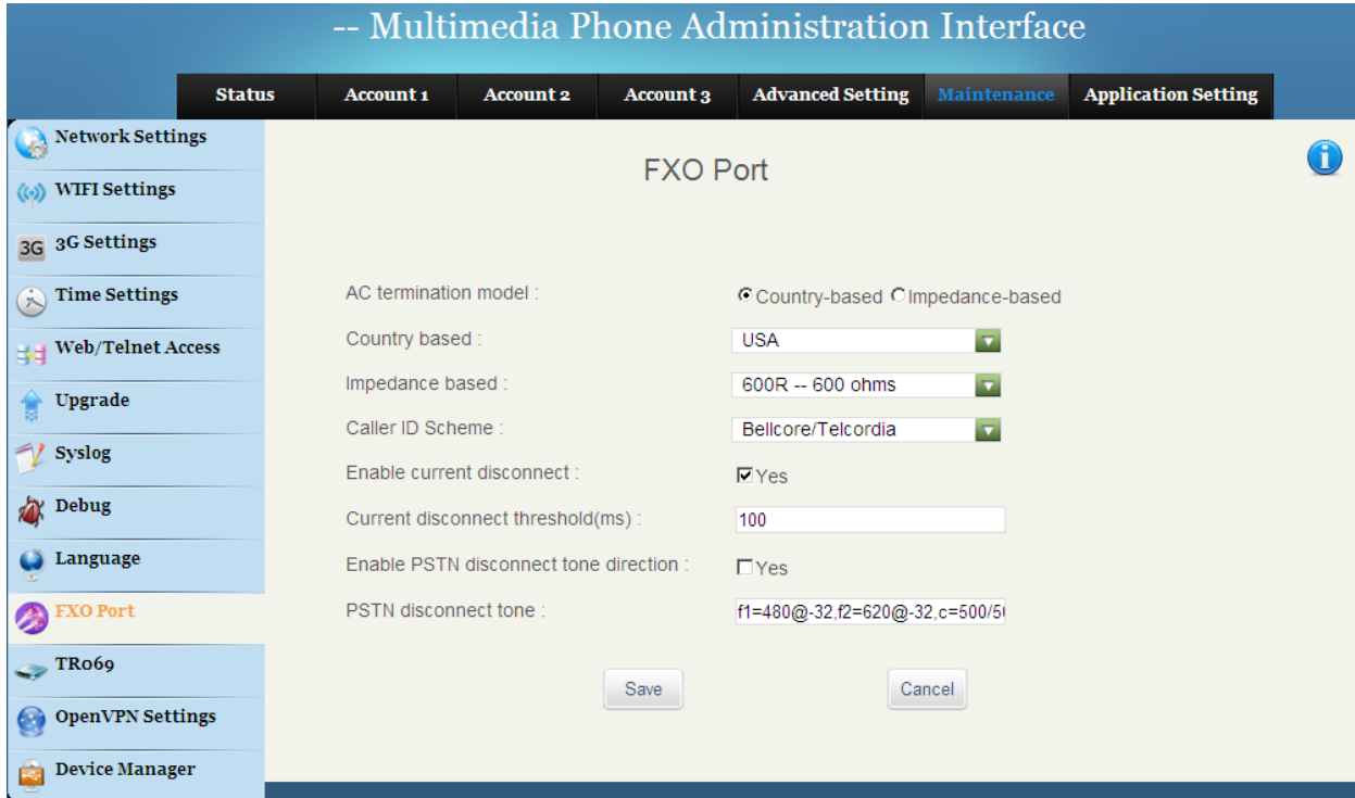
Figure: FXO Port Web UI Configuration
